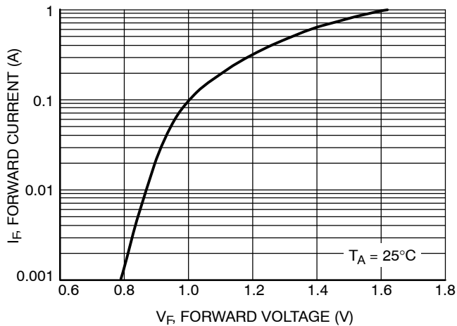
Figure 7. Forward Voltage
